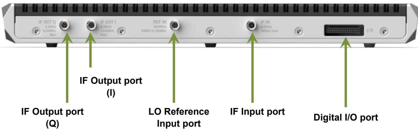
Rear view
